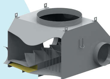
Control chambers
