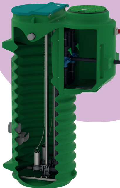
Community pumping stations
