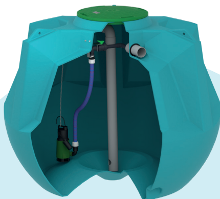
Large capacity regulation tanks
