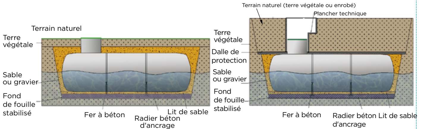
Pose standard
